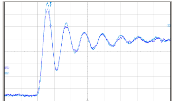
Ch 1: Co-axial shunt - DC-800MHz – 10mV/div Ch 2: CWTMini50HF 3 (100mm) - 12.8ns DE-SKEW Time base: 20ns/div
