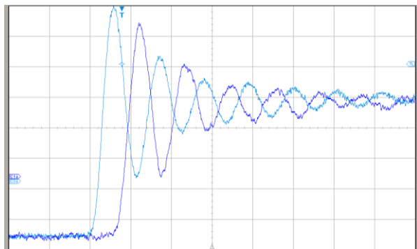
Ch 1: Co-axial shunt - DC-800MHz – 10mV/div Ch 2: CWTMini50HF 3 (100mm) - 5mV/div (0.5A/div) Time base: 20ns/div
