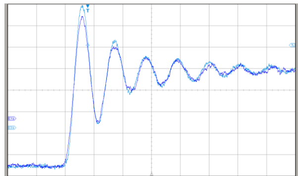
Ch 1: Co-axial shunt - DC-800MHz – 10mV/div Ch 2: CWTMini50HF 3 (100mm) - 12.8ns DE-SKEW Time base: 20ns/div
