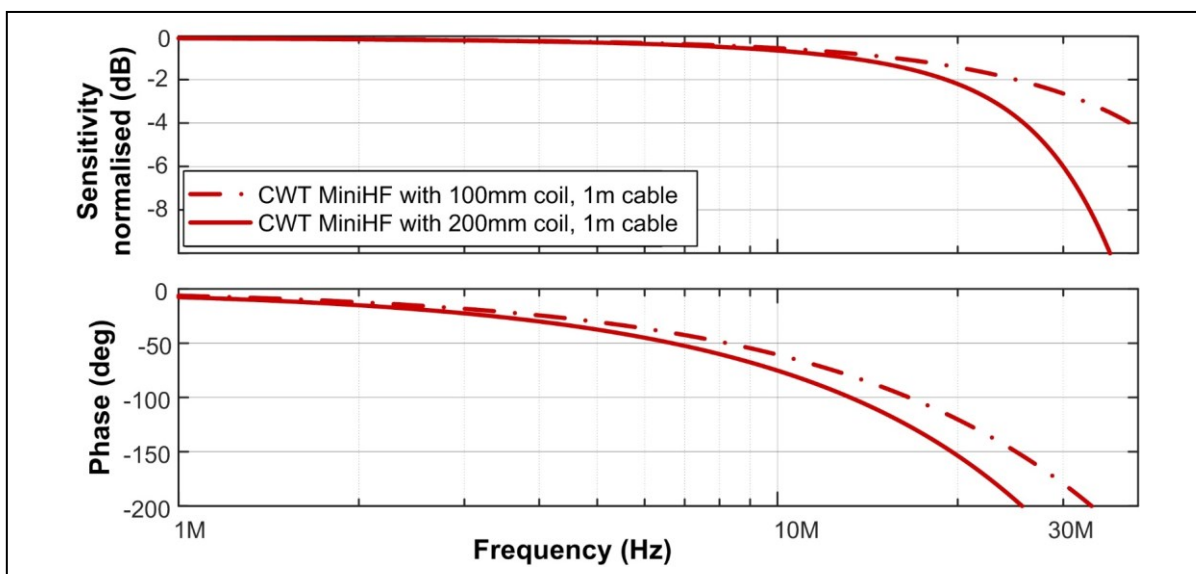
Figure 1. High frequency performance CWT MiniHF, 1m cable, 100 and 200mm coil
