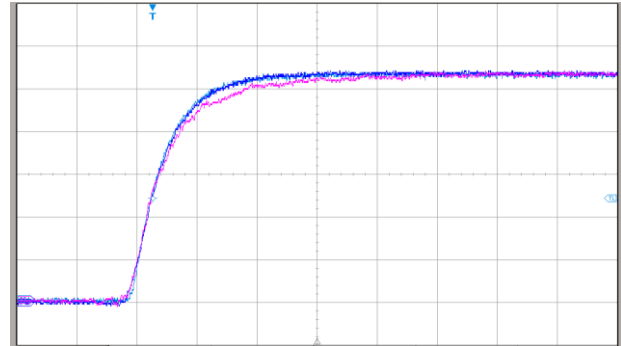
Ch 1: Co-axial shunt - DC-2GHz – 200mV/div Ch 2: CWTMiniHF 6 (100mm) – 24.7ns DE-SKEW Ch 3: CWTMini 6 (100mm) – 28.8ns DE-SKEW Time base: 50ns/div
