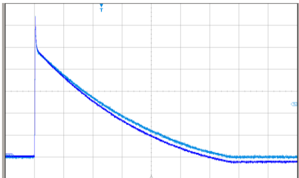
Ch 1: Co-axial shunt - DC-800MHz – 16.2mV/div Ch 2: CWTMiniHF 3 - 250mV/div (25A/div) – LF(-3dB) 11Hz Time base: 200μs/div
