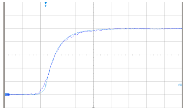
Ch 1: Co-axial shunt - DC-2GHz – 1V/div Ch 2: CWTMini50HF 3 (100mm) - 12.8ns DE-SKEW Time base: 10ns/div
