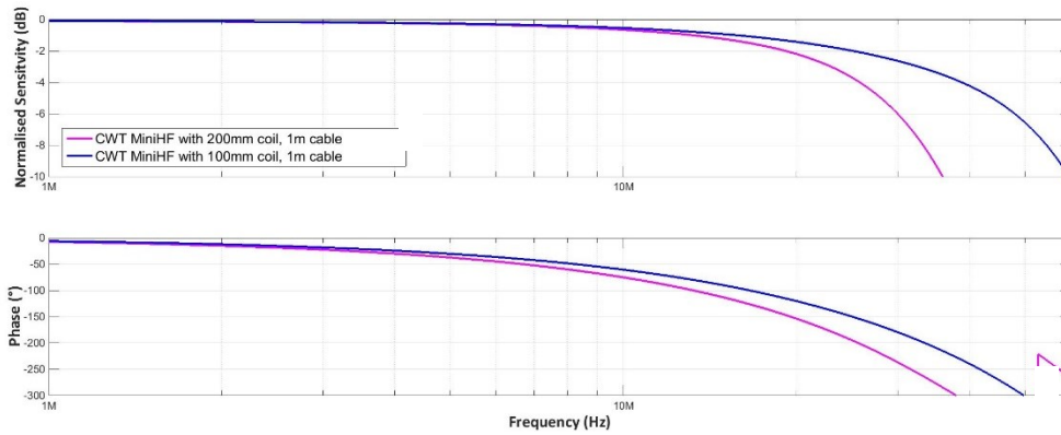
Appendix 2a. CWTMiniHF 1 / B / 1 / 100 / 5 (and 200mm) - Simulated frequency response for indication only
