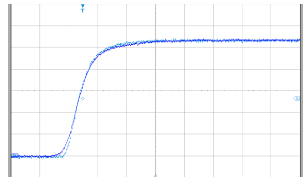
Ch 1: Co-axial shunt - DC-2GHz – 200mV/div Ch 2: CWTUM/1 – 16.8ns DE-SKEW - 400mV/div (20A/div) Time: 20ns/div
