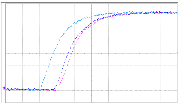
Ch 1: Co-axial shunt - DC-2GHz – 20mV/div Ch 2: CWTMiniHF 03 (100mm) - 205mV/div (2A/div) Ch 3: CWTMiniHF 03 (200mm) - 205mV/div (2A/div) Time base: 20ns/div
