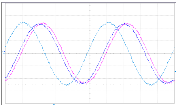
Ch 1: Co-axial shunt - DC-800MHz – 40mV/div Ch 2: CWTMiniHF 03 (100mm) - 200mV/div (2A/div) Ch 3: CWTMiniHF 03 (200mm) - 200mV/div (2A/div) Time base: 20ns/div
