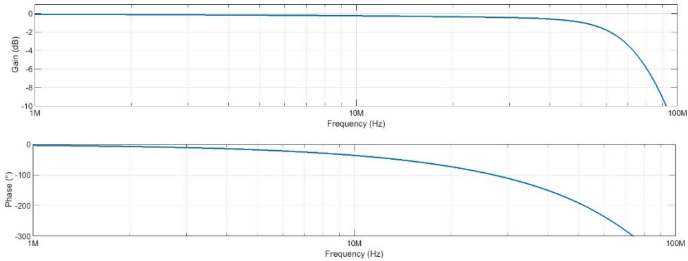
Appendix 4a. CWTMini50HF 3 / B / 1 / 100 / 2 - Simulated frequency response for indication only
