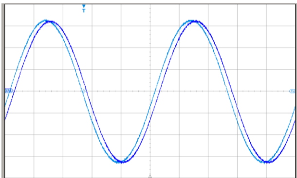
Ch 1: Co-axial shunt - DC-800MHz – 60mV/div (3A/div) Ch 2: CWTUM/1 - 60mV/div (3A/div) Time base: 100ns/div
