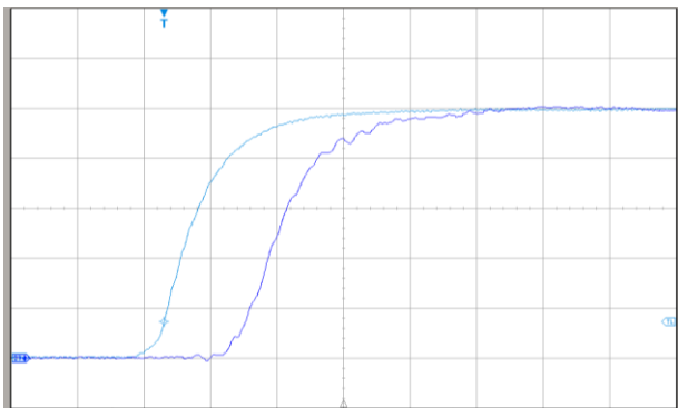
Ch 1: Co-axial shunt - DC-2GHz – 1V/div Ch 2: CWTMini50HF 3 (100mm) - 101mV/div (10A/div) Time base: 10ns/div
