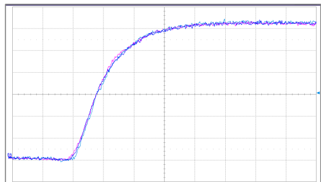
Ch 1: Co-axial shunt - DC-2GHz – 40mV/div Ch 2: CWTMiniHF 03 (100mm) - 17.5ns DE-SKEW Ch 3: CWTMiniHF 03 (200mm) - 20.9ns DE-SKEW Time base: 20ns/div
