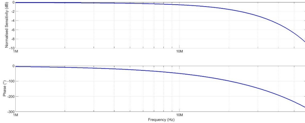
Appendix 1a. CWTUM 1/B/1/80 Simulated frequency response for indication only
