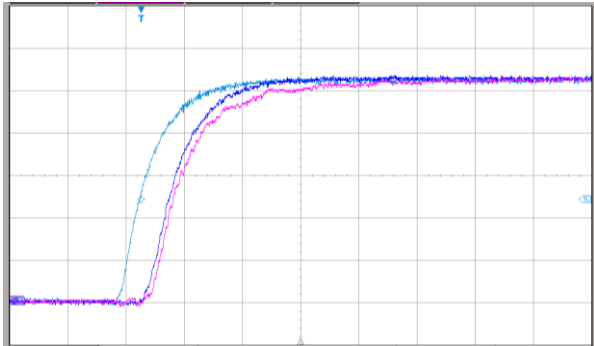
Ch 1: Co-axial shunt - DC-2GHz – 200mV/div Ch 2: CWTMiniHF 6 (100mm) - 100mV/div (20A/div) Ch 3: CWTMini 6 (100mm) - 100mV/div (20A/div) Time base: 50ns/div
