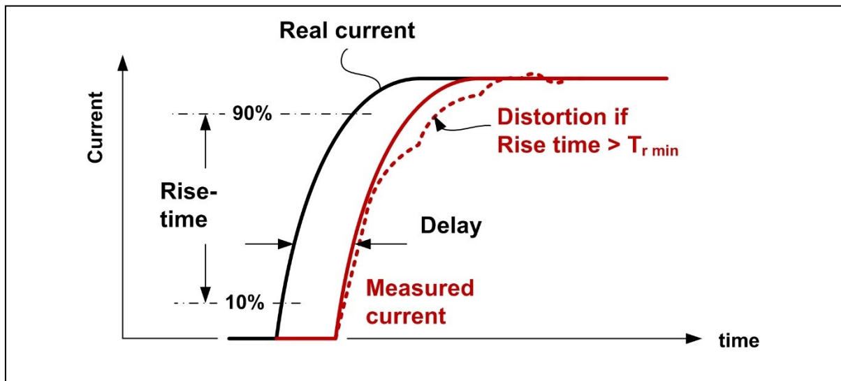
Figure 2. Rise time and Delay definitions
