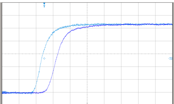
Ch 1: Co-axial shunt - DC-2GHz – 200mV/div Ch 2: CWTUM/1 - 400mV/div (20A/div) Time: 20ns/div
