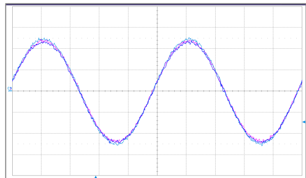
Ch 1: Co-axial shunt - DC-800MHz – 40mV/div Ch 2: CWTMiniHF 03 (100mm) - 17.5ns DE-SKEW Ch 3: CWTMiniHF 03 (200mm) - 20.9ns DE-SKEW Time base: 20ns/div
