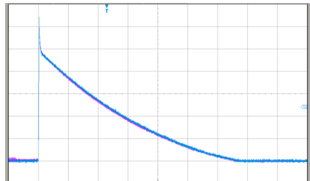
Ch 1: Co-axial shunt - DC-800MHz – 40mV/div Ch 3: CWTMiniHF 3 - 250mV/div (25A/div) – LF(-3dB) 2.3Hz Time base: 200μs/div
